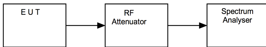
Figure iv Test Setup
