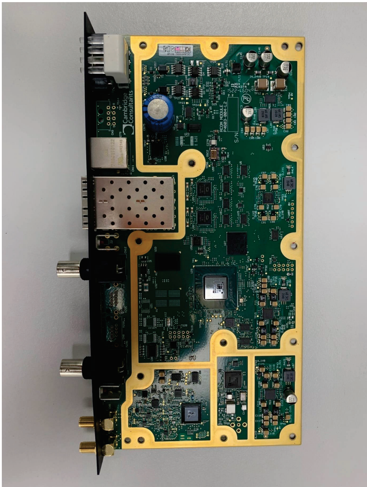
Internal PCB top
