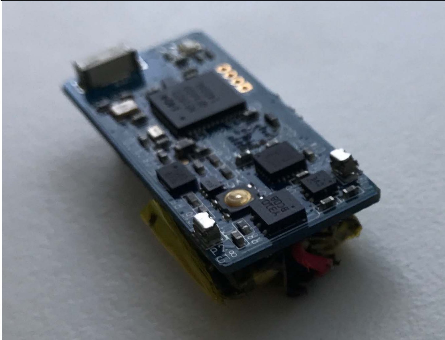
Top/End View With Battery Wiring
