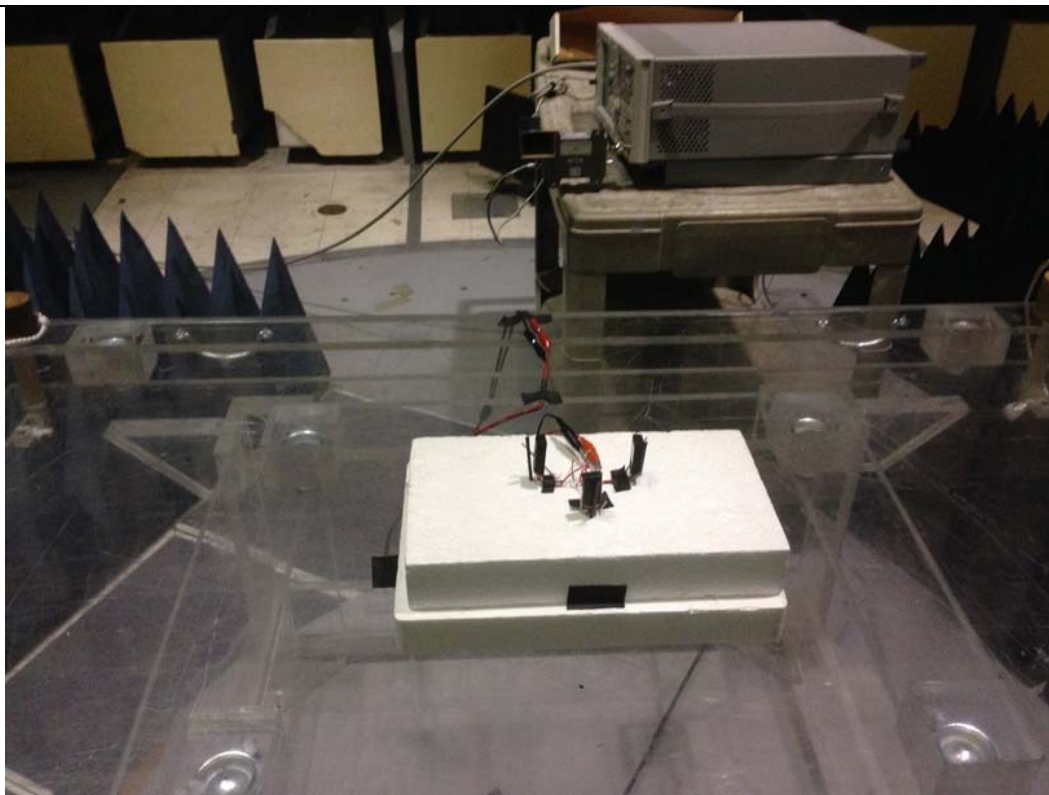
Spurious Front
