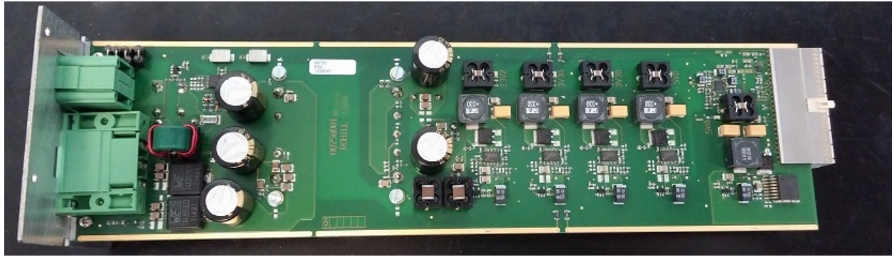
PSU TOP VIEW
