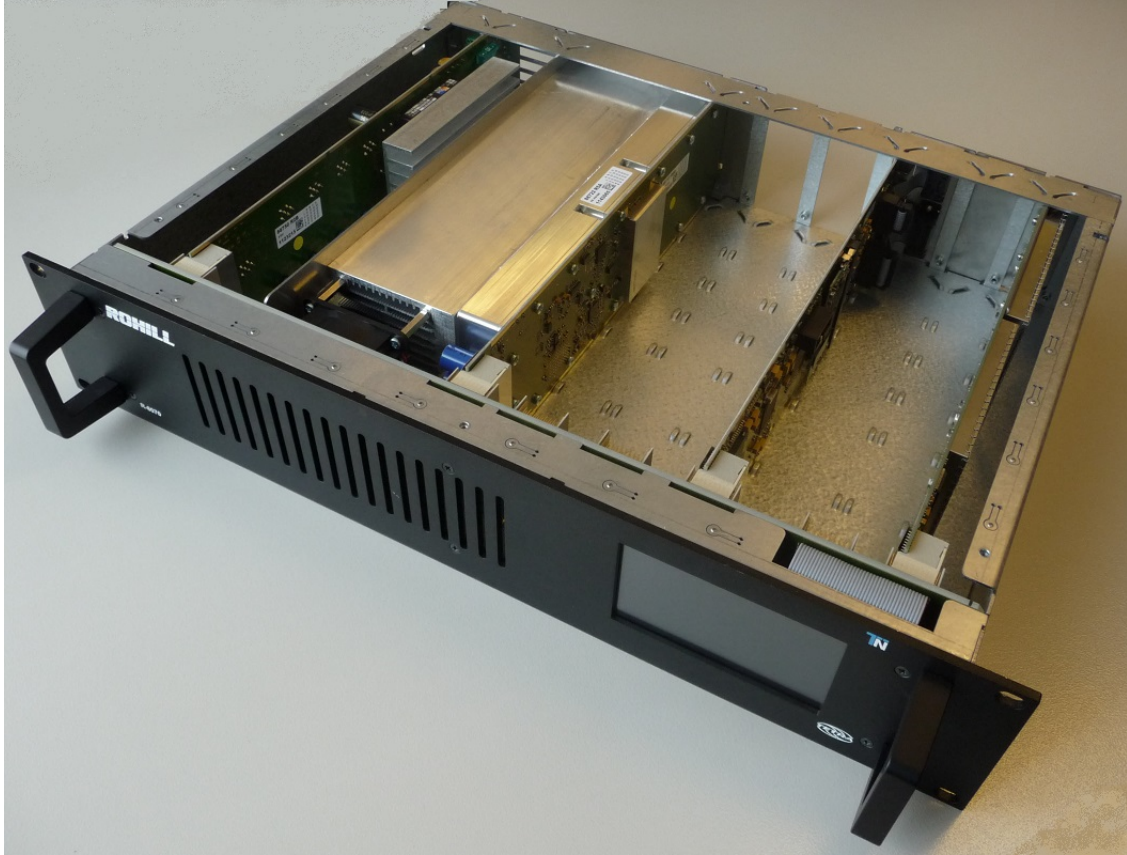
INTERNAL TOP SIDE
