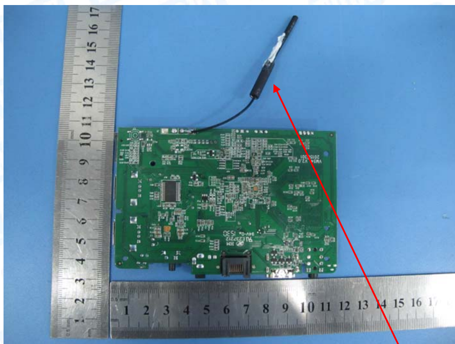
2.4G Embedded Antenna
