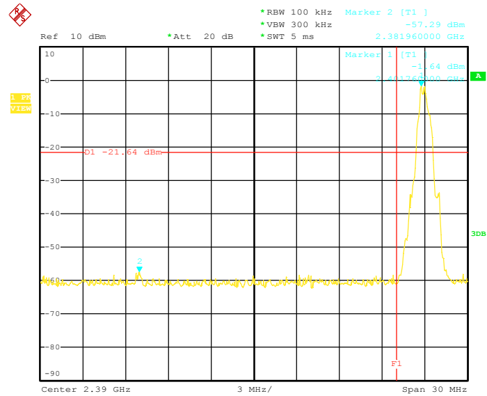
Bluetooth 4.1 LE Channel: Low
