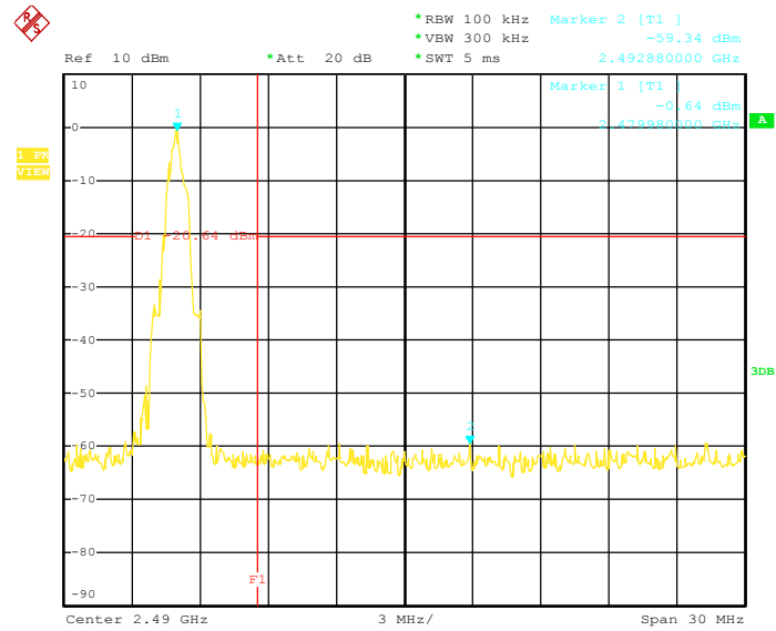
Bluetooth 4.0 LE Channel: High
