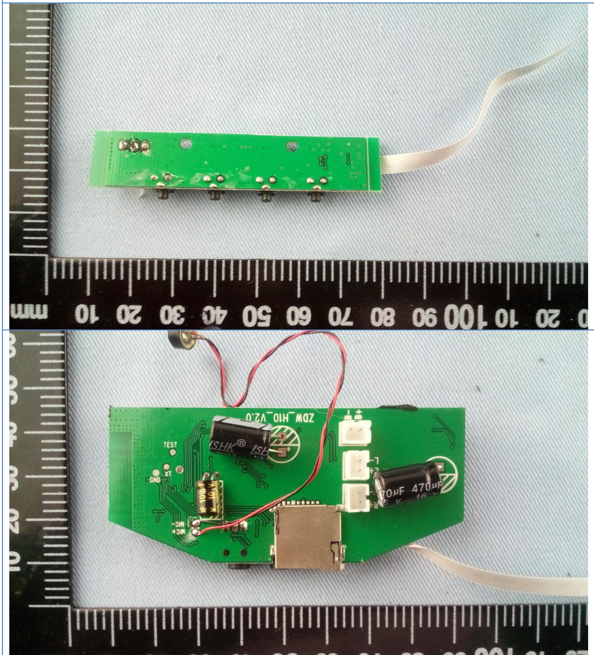
Main board solder side
