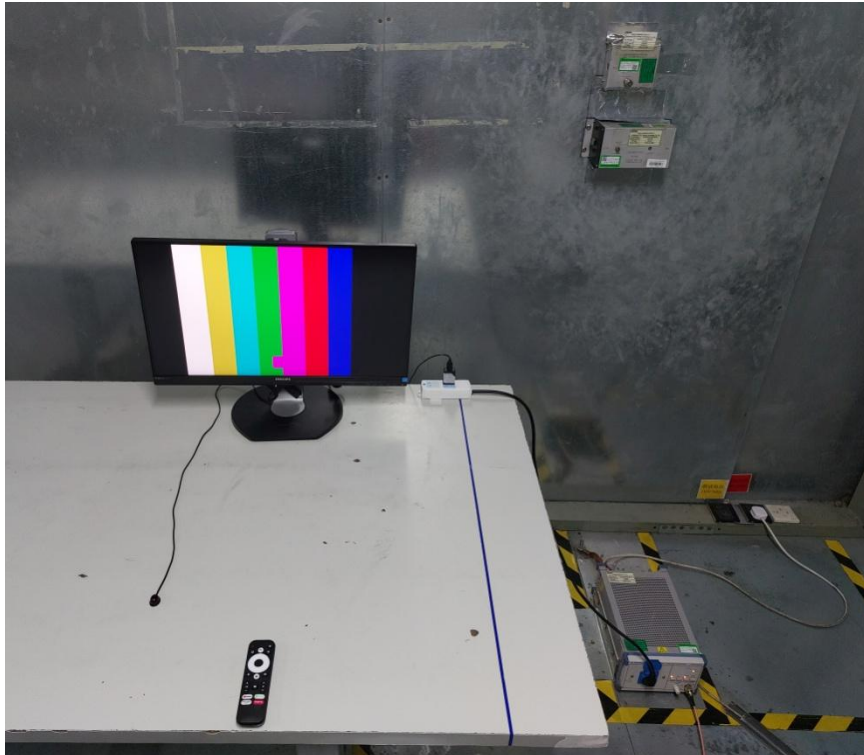
AC Conducted Measurement Photos
