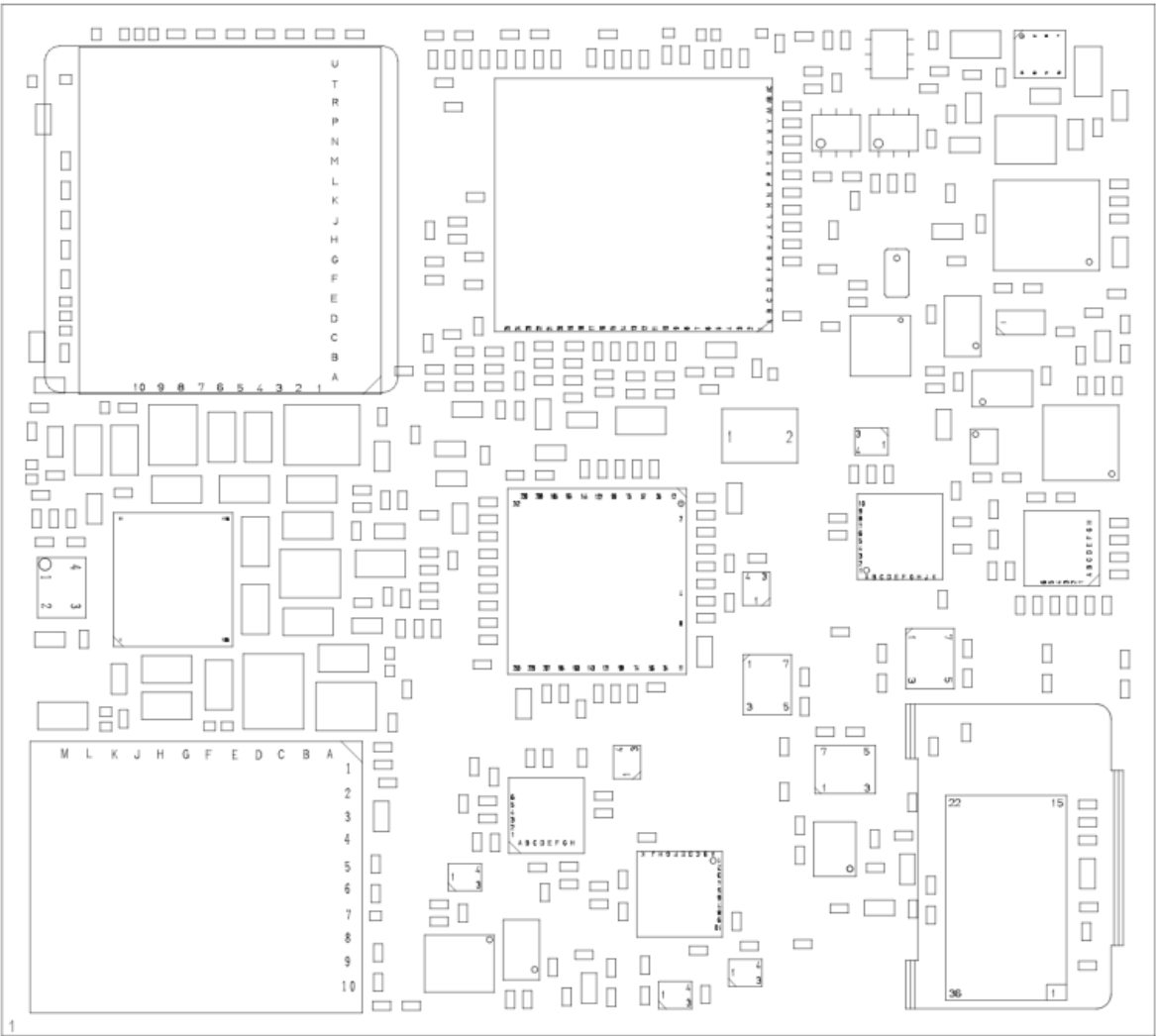
Figure 2: Floorplan ALAS5V-US
