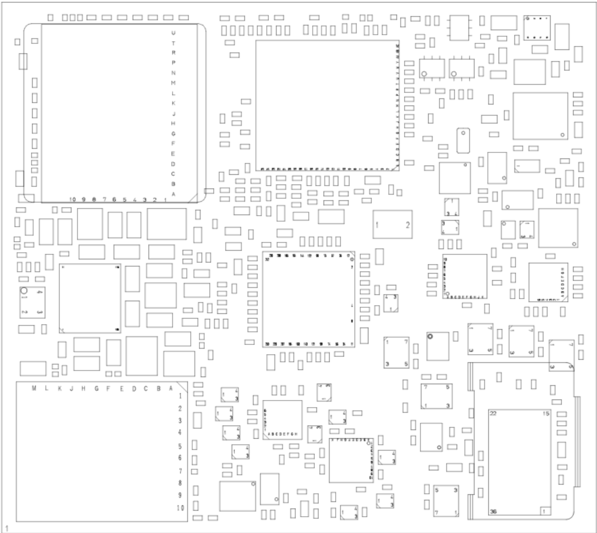
Figure 1: Floorplan ALAS5-AM
