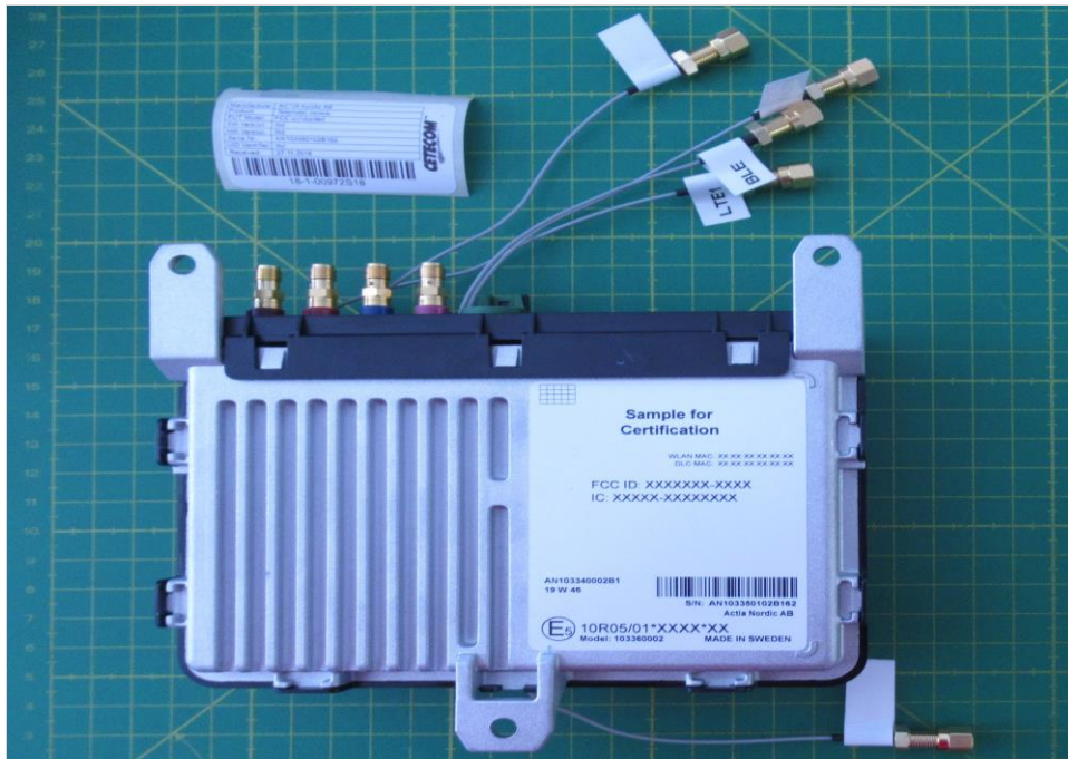
Photograph 7: EUT B_Rear side view
