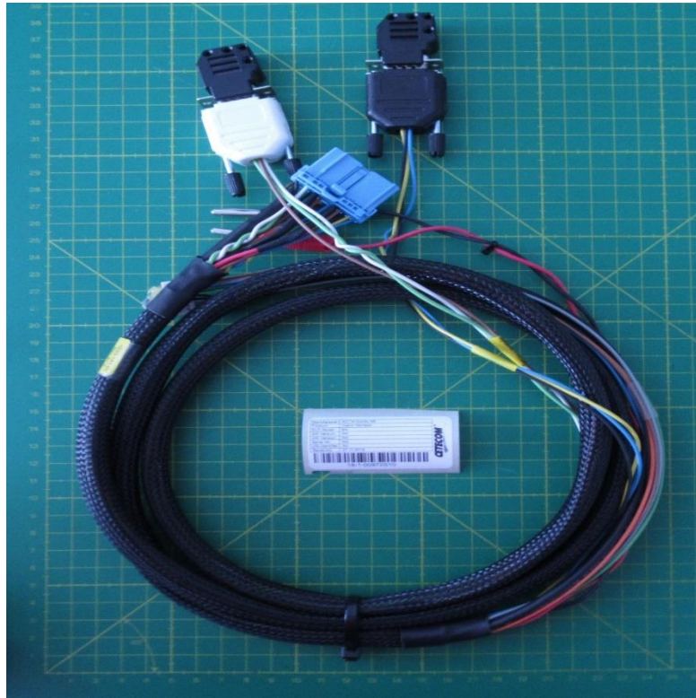
Photograph 7: AE1
