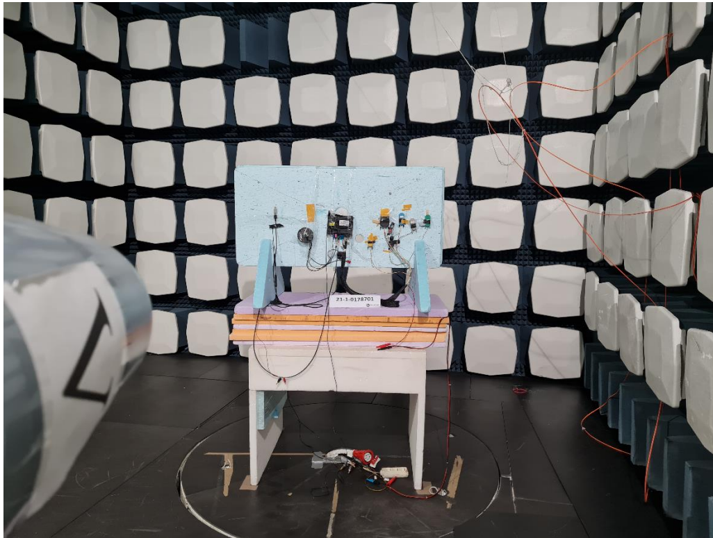
Fig. Mea.: 3 : Radiated measurement Overall view
