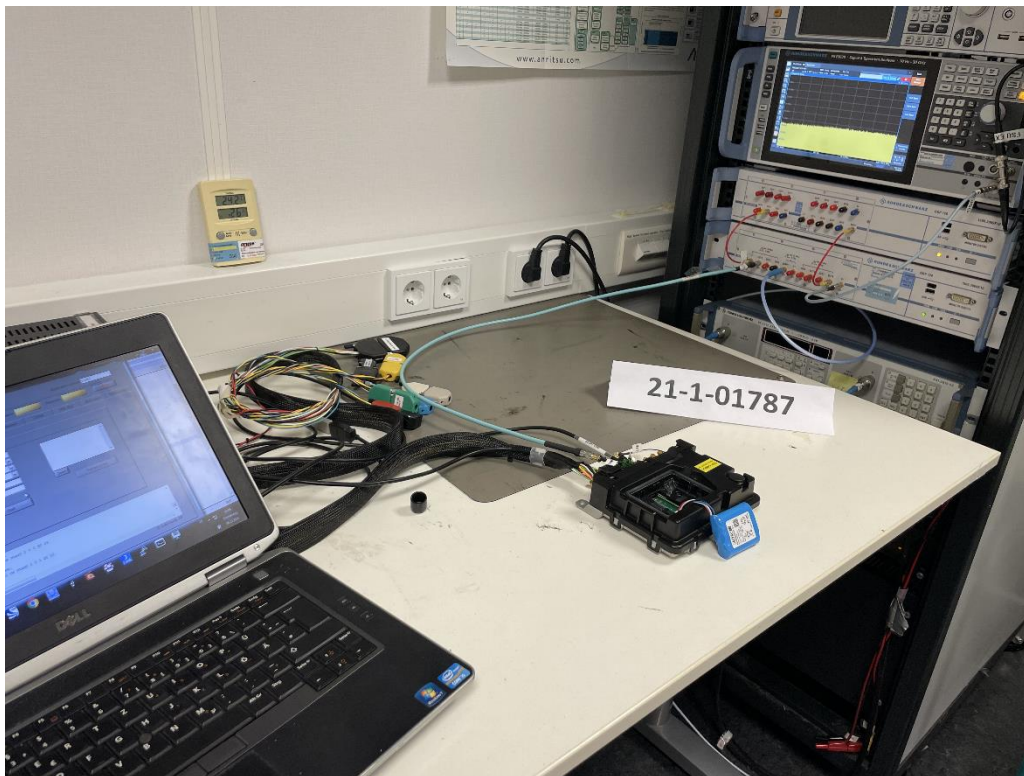
Fig. Mea.: 1 : Conducted measurement Overall view
