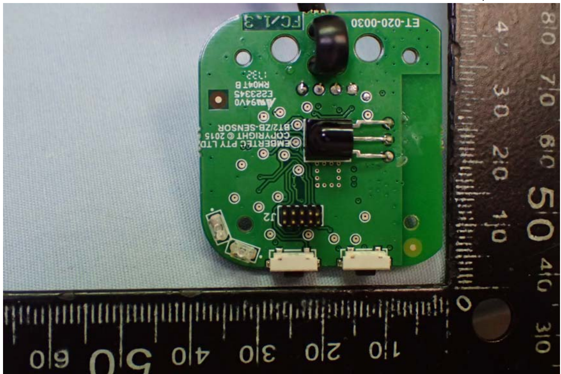
Figure 6 Main Board, Front View
