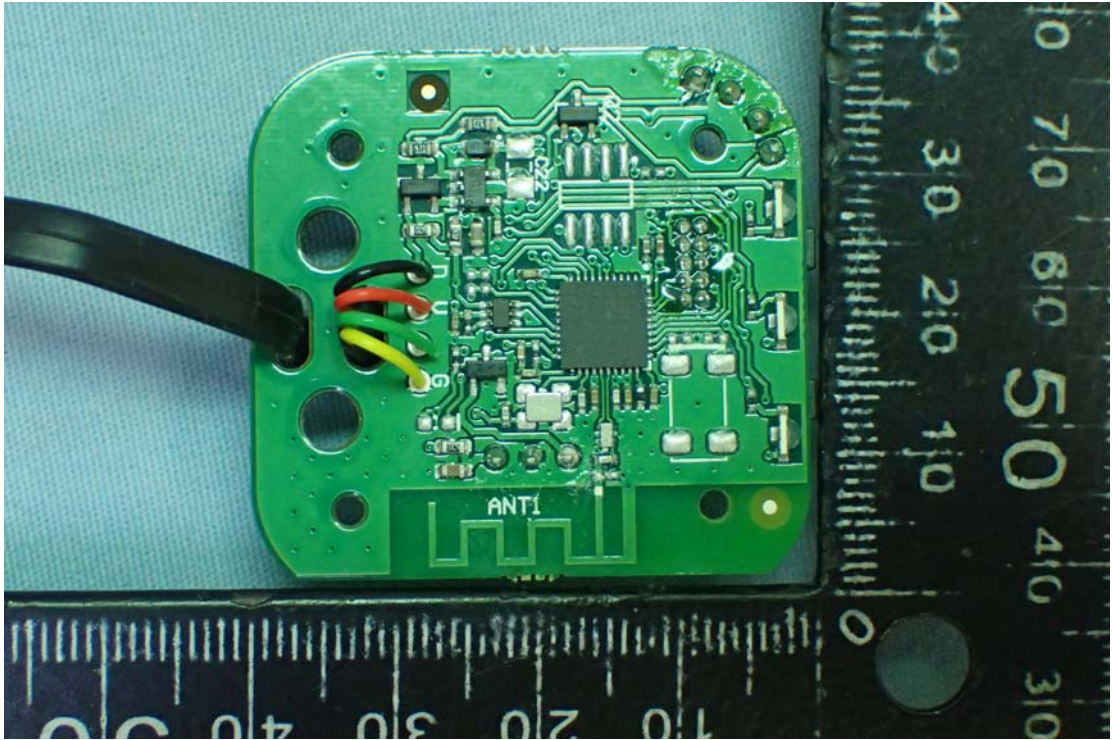
Figure 7 Main Board, Back View
