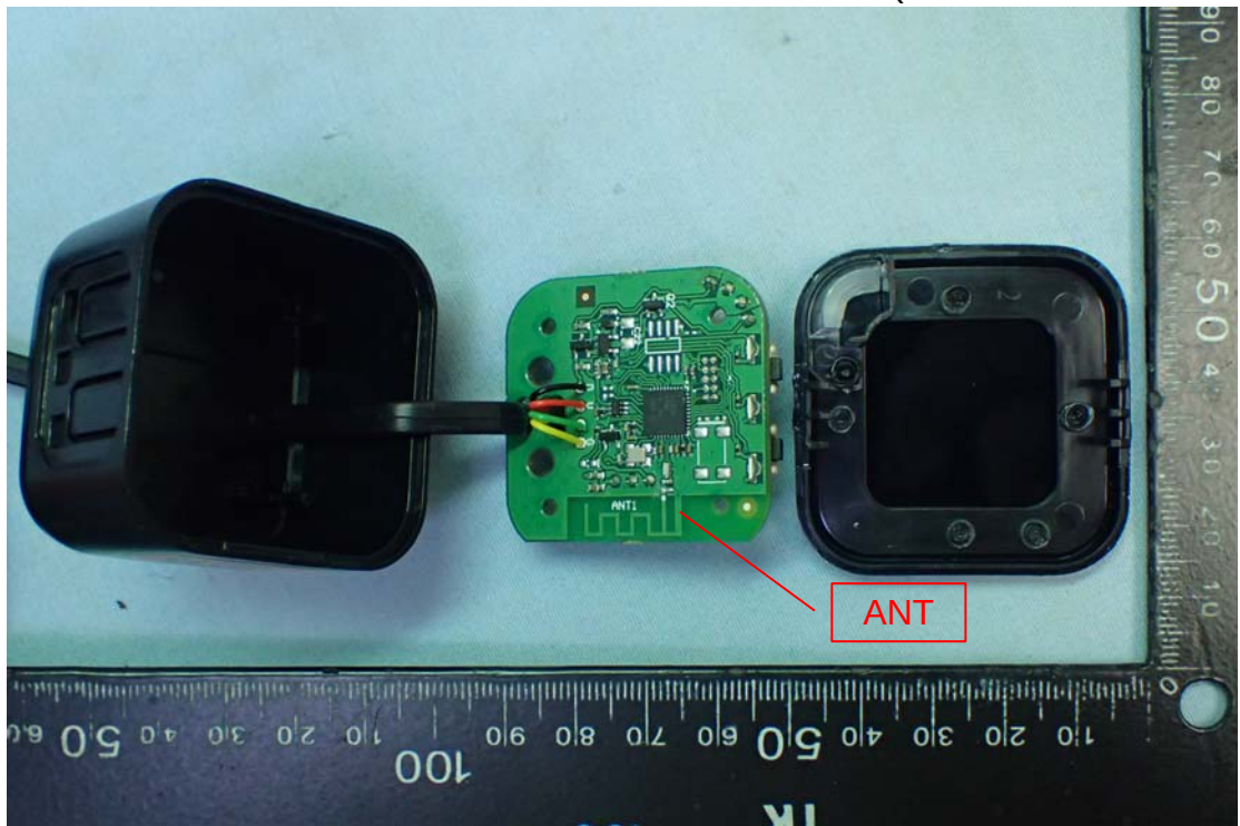
Figure 5 Internal View (Remove Cover View)
