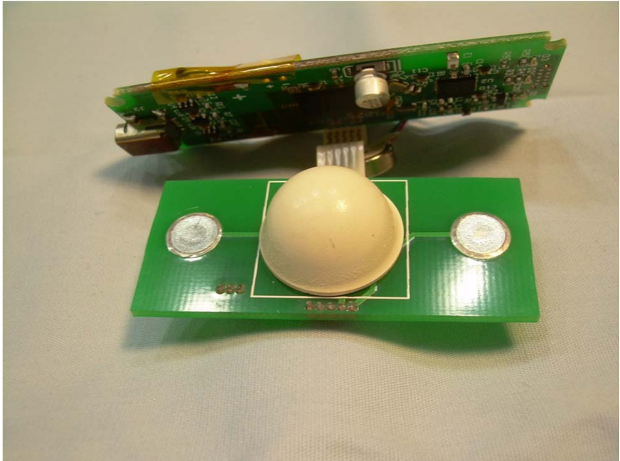
View of the Bottom Side of the Contact PCB
