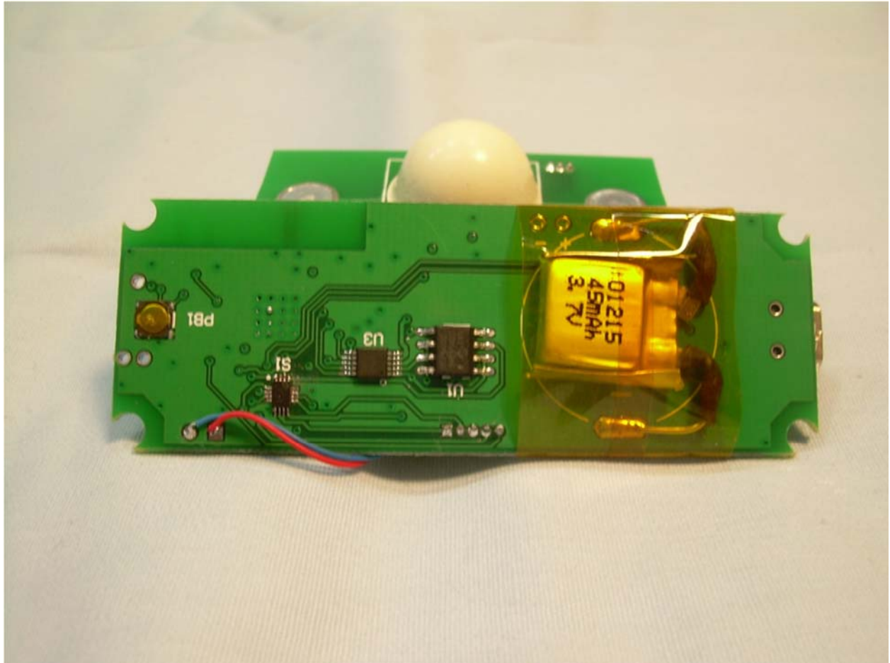
View of the Battery Side of the Main PCB
