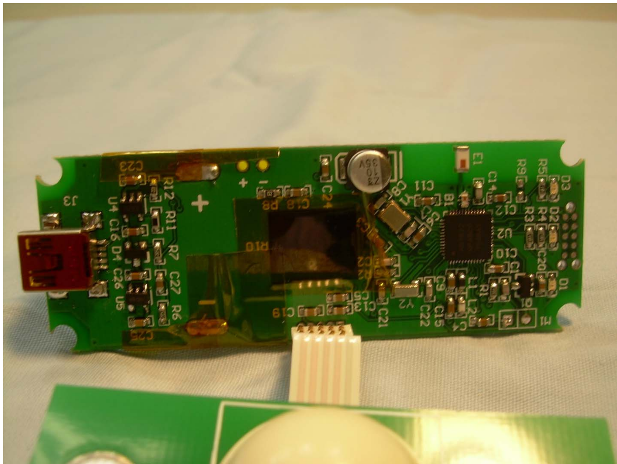
Photograph 13 – View of the Top Side of the Main PCB
