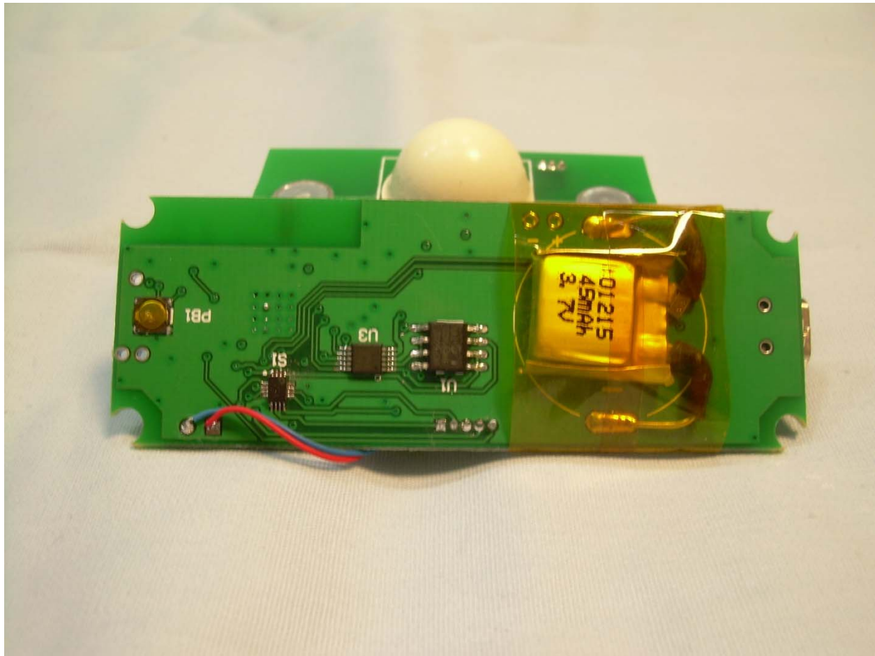
Photograph 14 – View of the Battery Side of the Main PCB
