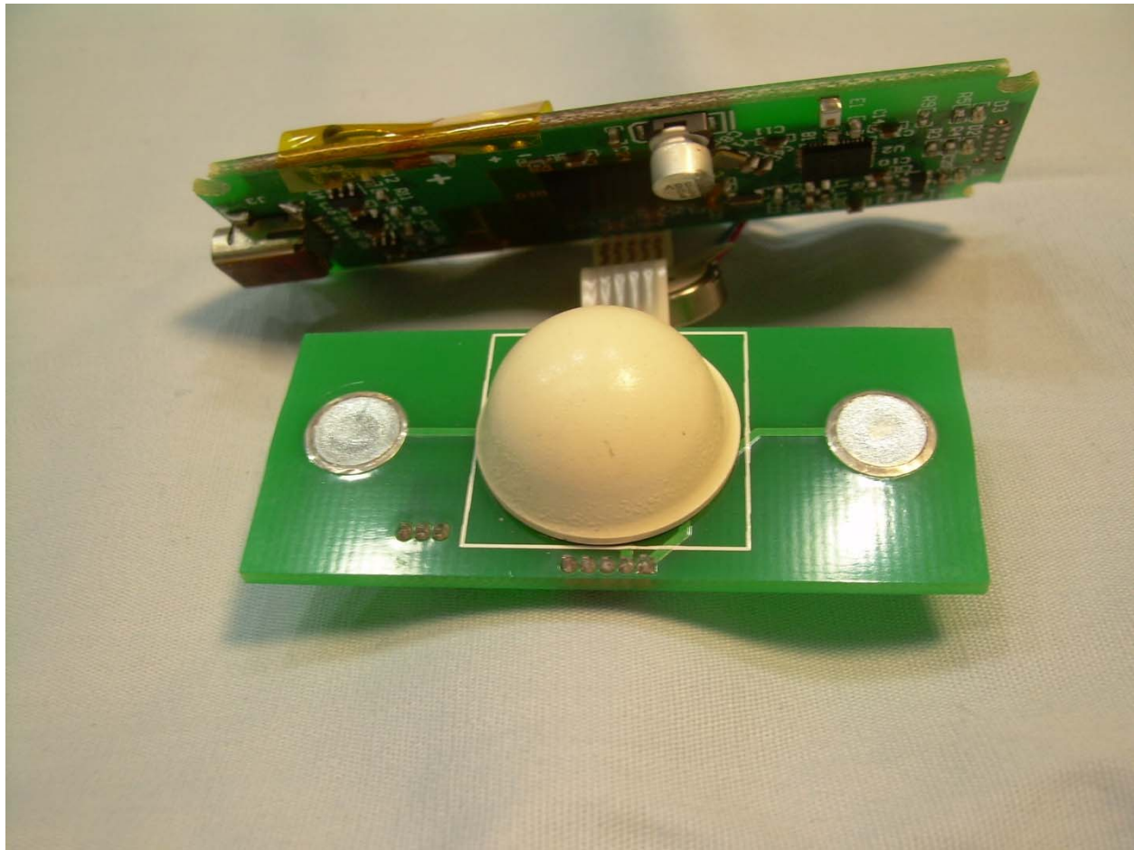
Photograph 12 – View of the Bottom Side of the Contact PCB
