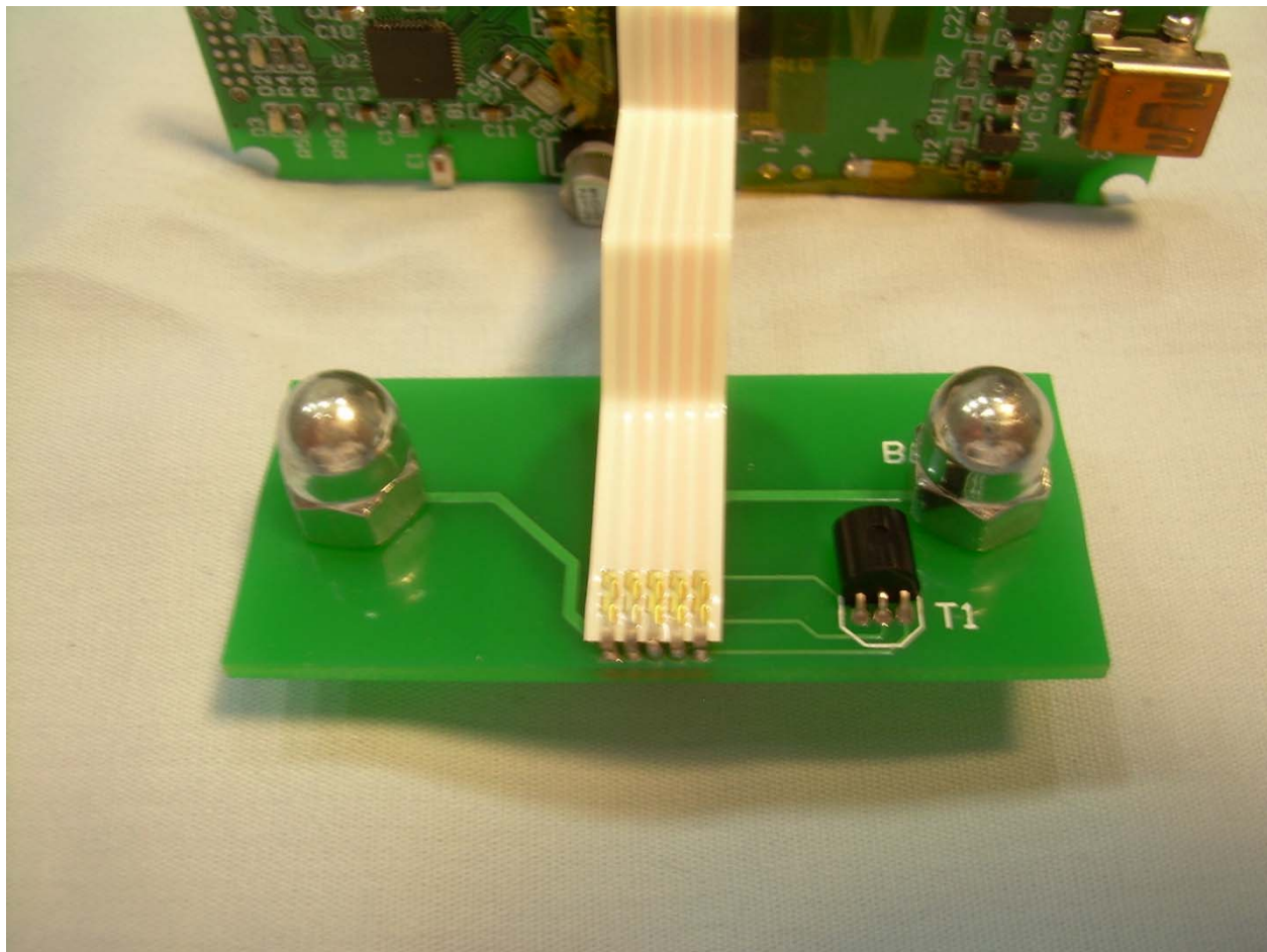
Photograph 11 – View of the Top Side of the Contact PCB
