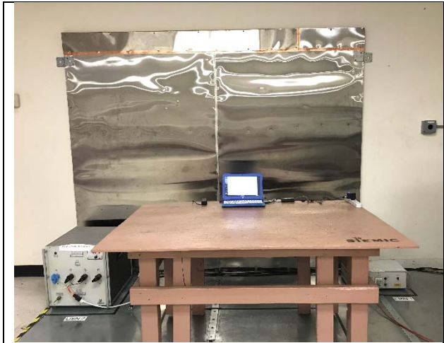
AC Line Conducted Emissions – Front View
