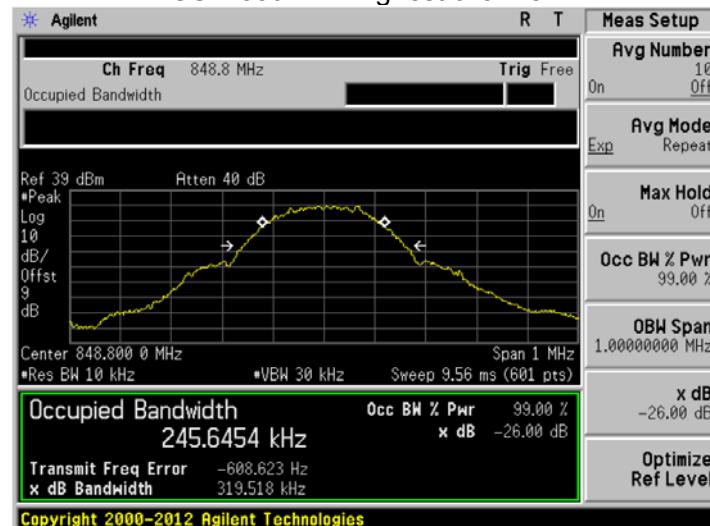
GSM 850MHz Highest channel:
