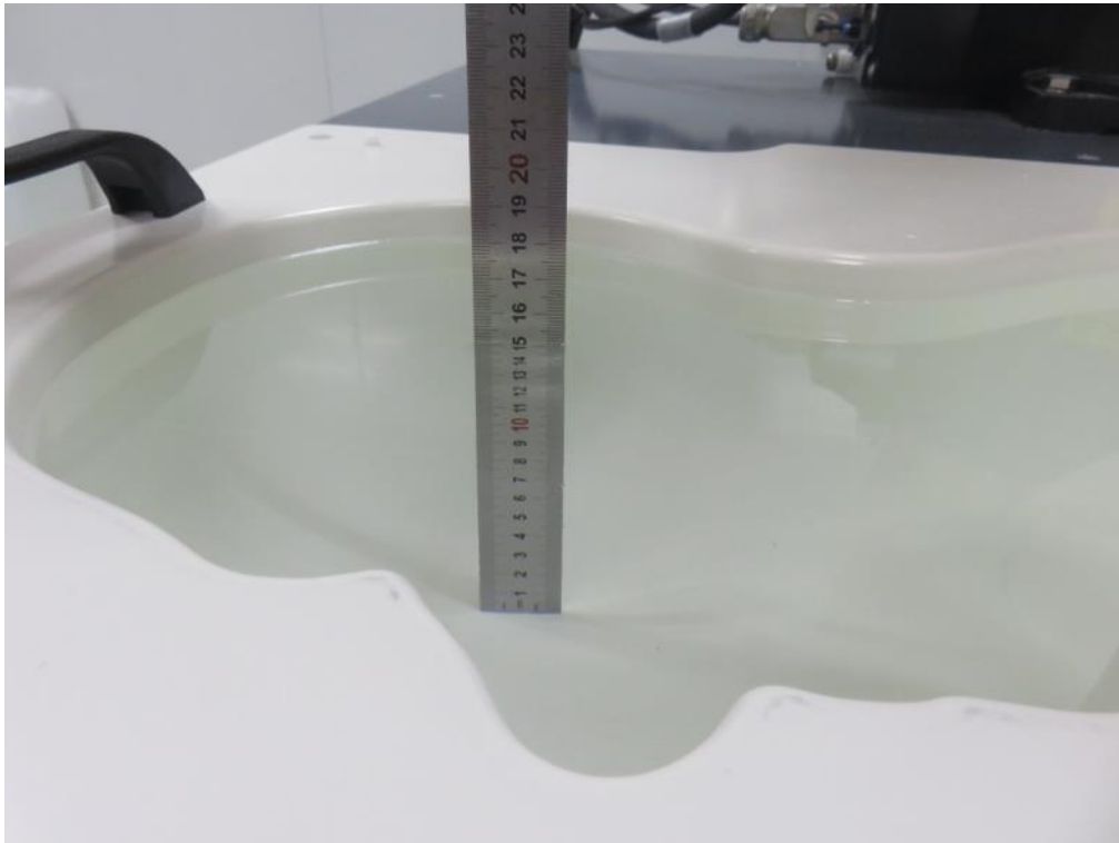
Photograph of the depth in the Head Phantom (750MHz, 15.2cm depth)
