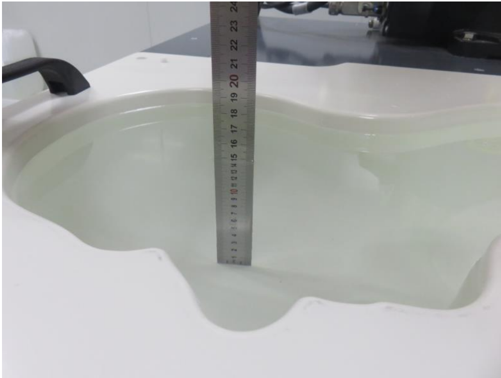
Photograph of the depth in the Head Phantom (1800MHz, 15.1cm depth)
