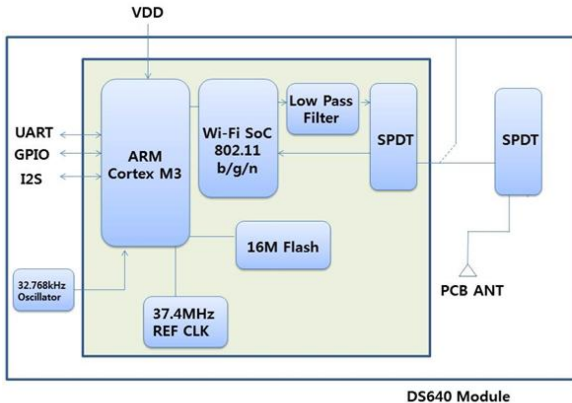
FIGURE 2: DS640 Block Diagram
