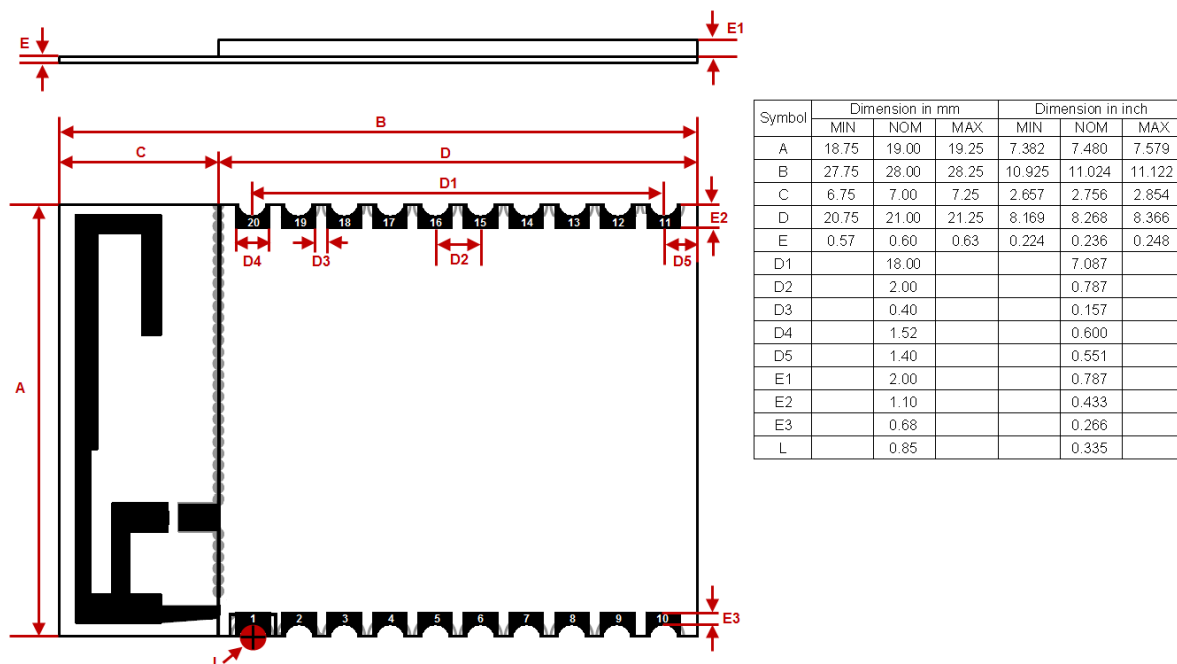
Figure 6.2. DS640 Recommended Footprint (Top View)
