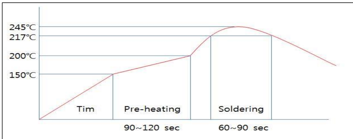
Figure 6.3 : DS640 Recommended Reflow Profile
