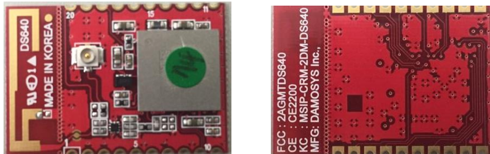
Figure 6.1 : DS640 General view
