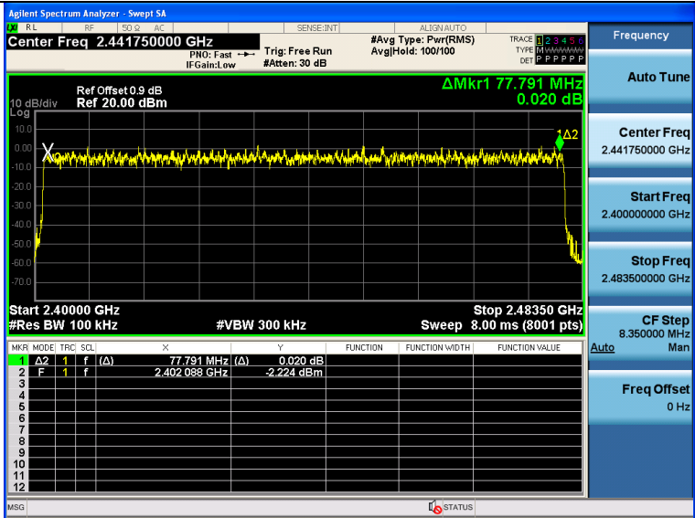
π/4DQPSK Modulation
