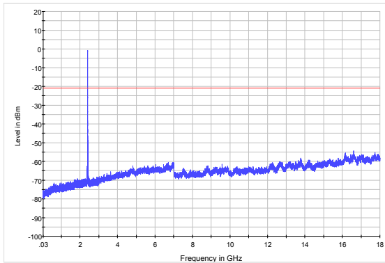
Zigbee CH18 30MHz to 18GHz
