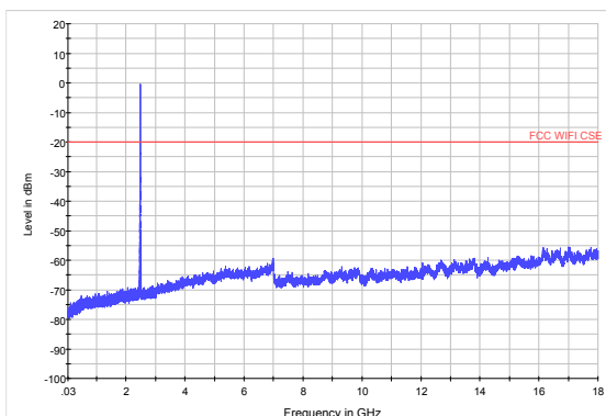
Zigbee CH26 30MHz to 18GHz
