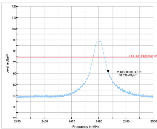
Zigbee-Channel 26: Peak
