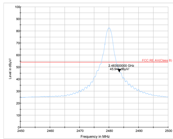
Zigbee-Channel 26: Average
