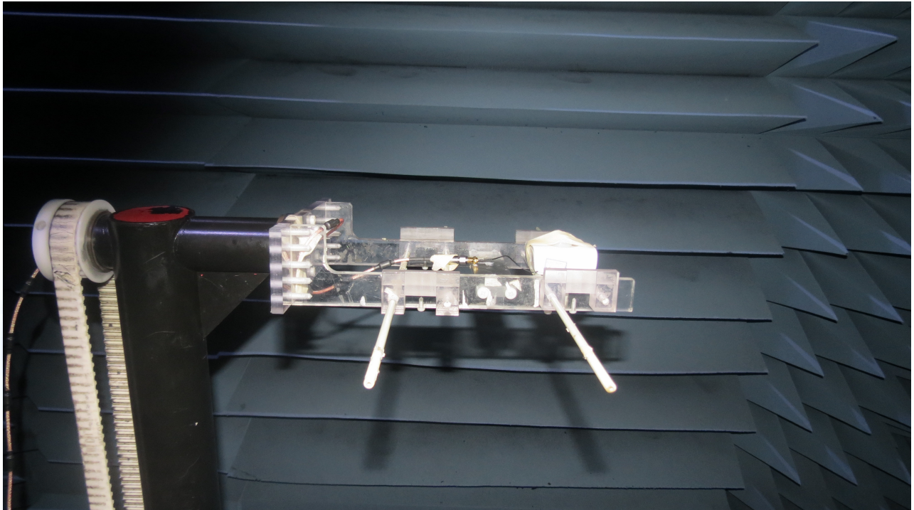
Picture 2 Test Setup
