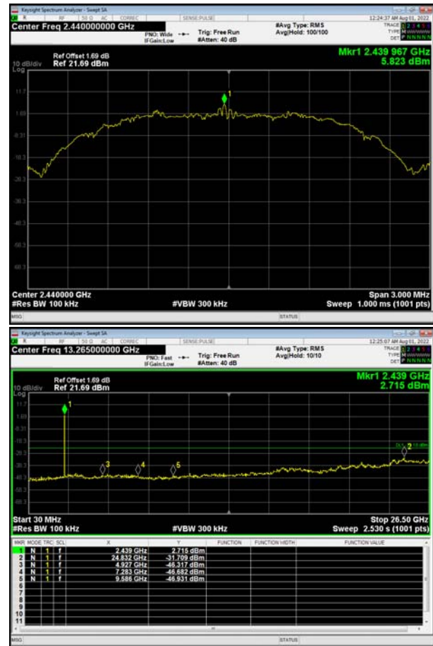
Zigbee CH18
