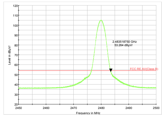
Zigbee-Channel 26: Average
