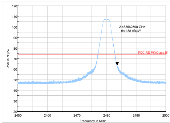
Zigbee-Channel 26: Peak
