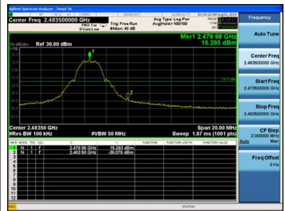
Zigbee, Channel No.: 26
