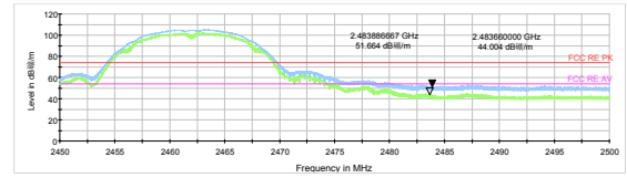
802.11b-Channel 11 Peak+ Average
