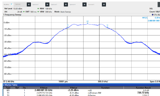
Figure 8.4-3: Minimum 6 dB bandwidth, GFSK, 1 Mbps, 2480 MHz
