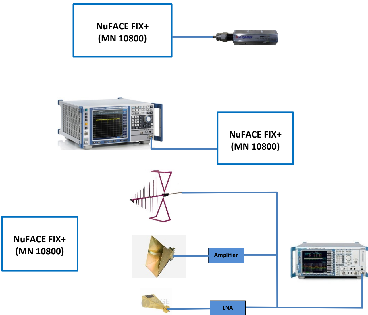
Figure 3.6-1: Test setup diagram
