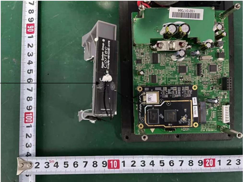
Wi-Fi/ Bluetooth Antenna 2
