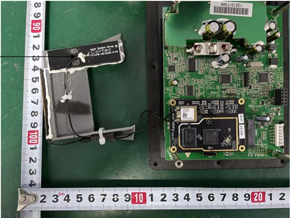
Wi-Fi/ Bluetooth Antenna 1
