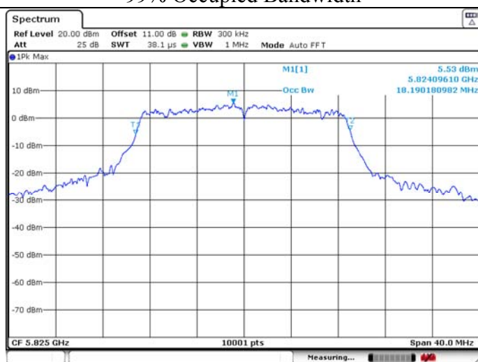
99% Occupied Bandwidth
