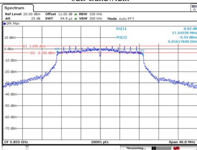
6dB Bandwidth
