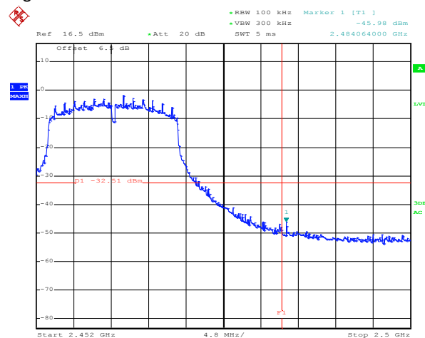
802.11g
