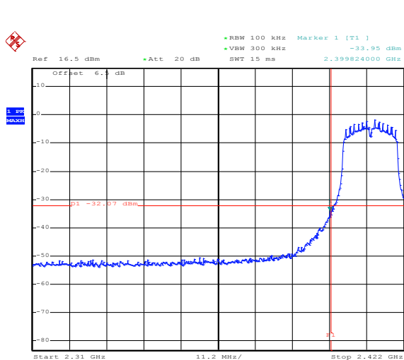
802.11g
