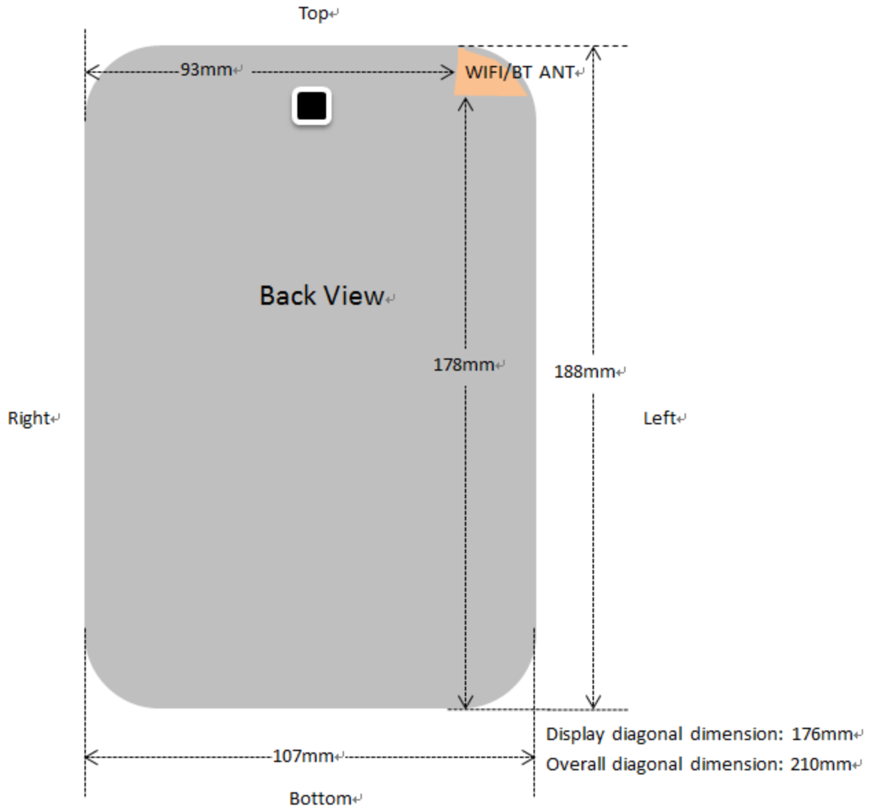
Fig.14.1 EUT Antenna Locations
