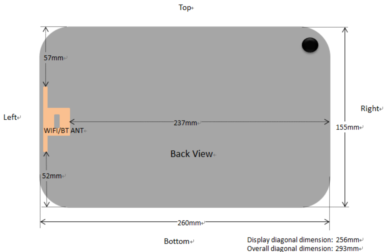
Fig.14.1 EUT Antenna Locations
