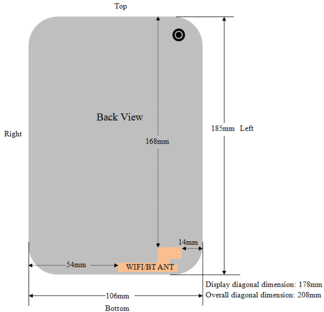
Fig.14.1 EUT Antenna Locations
