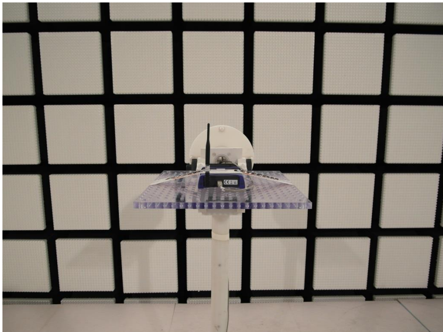
Photo 4: Receiver
