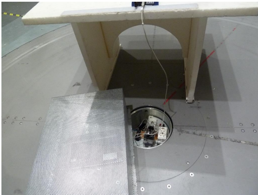
Photo 7: Receiver
