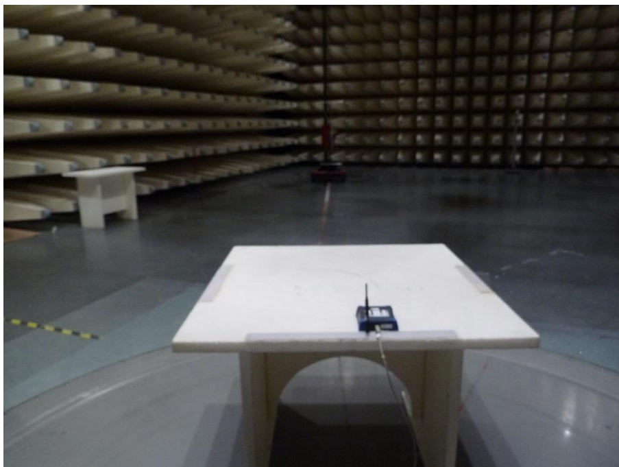
Photo 6: Receiver
