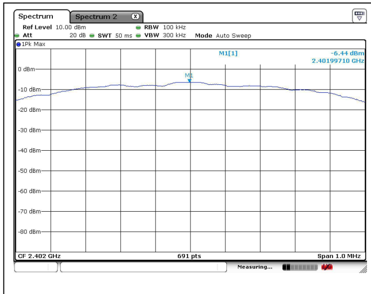
Lower channel
