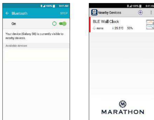
Android Version
