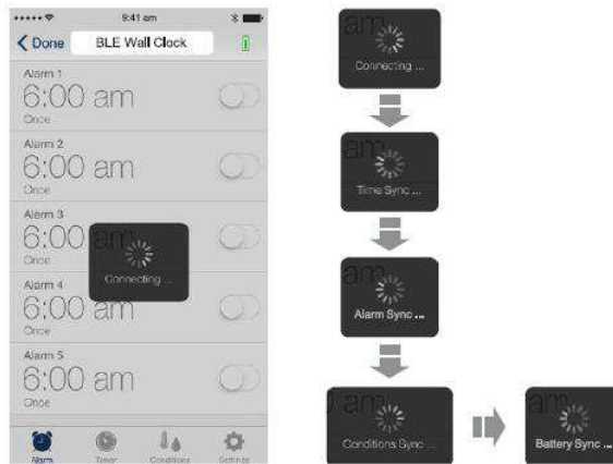
iOS Version
