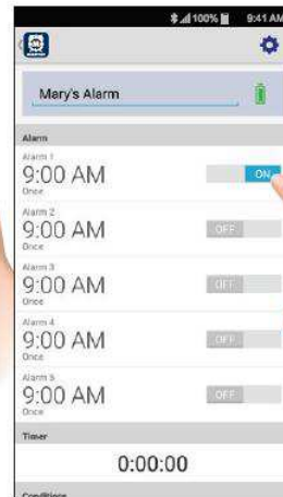
Android Version
