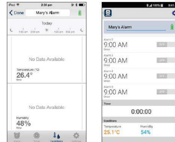
iOS Version
