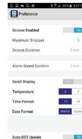
Android Version
