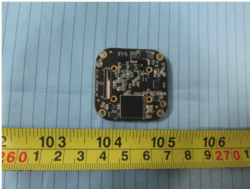
EUT – Pan-Tilt Main Board 2 Top View
