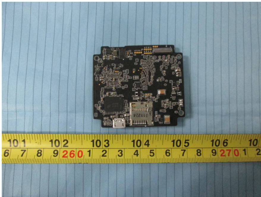
EUT – Pan-Tilt Main Board 1 Top View
