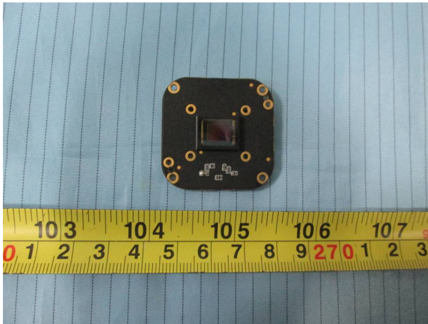
EUT – Pan-Tilt Main Board 2 Bottom View
