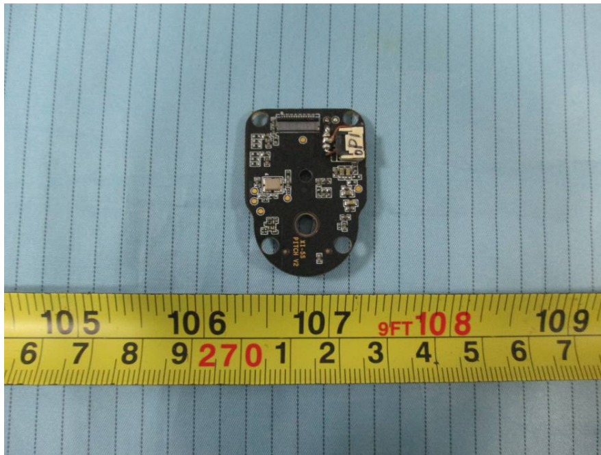
EUT – Pan-Tilt Main Board 4 Bottom View
