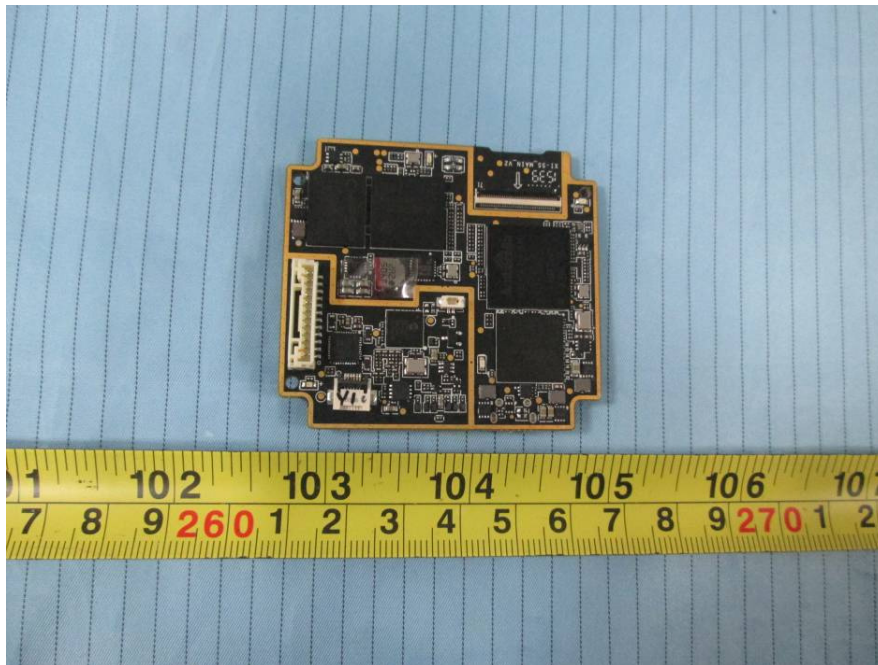
EUT – Pan-Tilt Main Board 1 Bottom View
