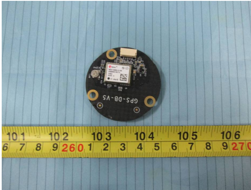
EUT – GPS Main Board Top View
