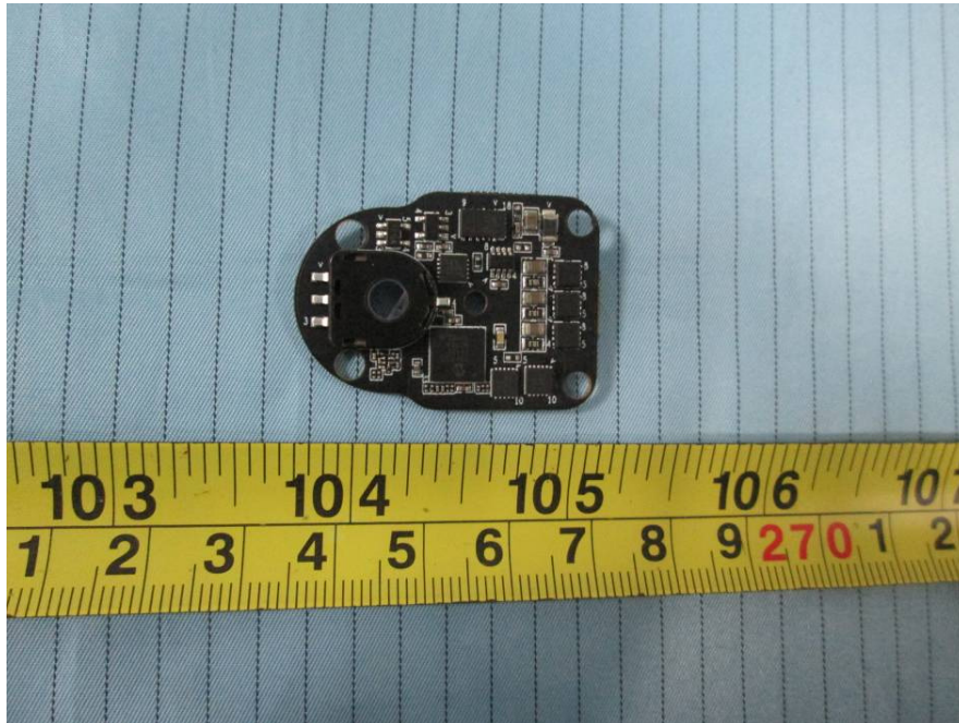
EUT – Pan-Tilt Main Board 3 Bottom View
