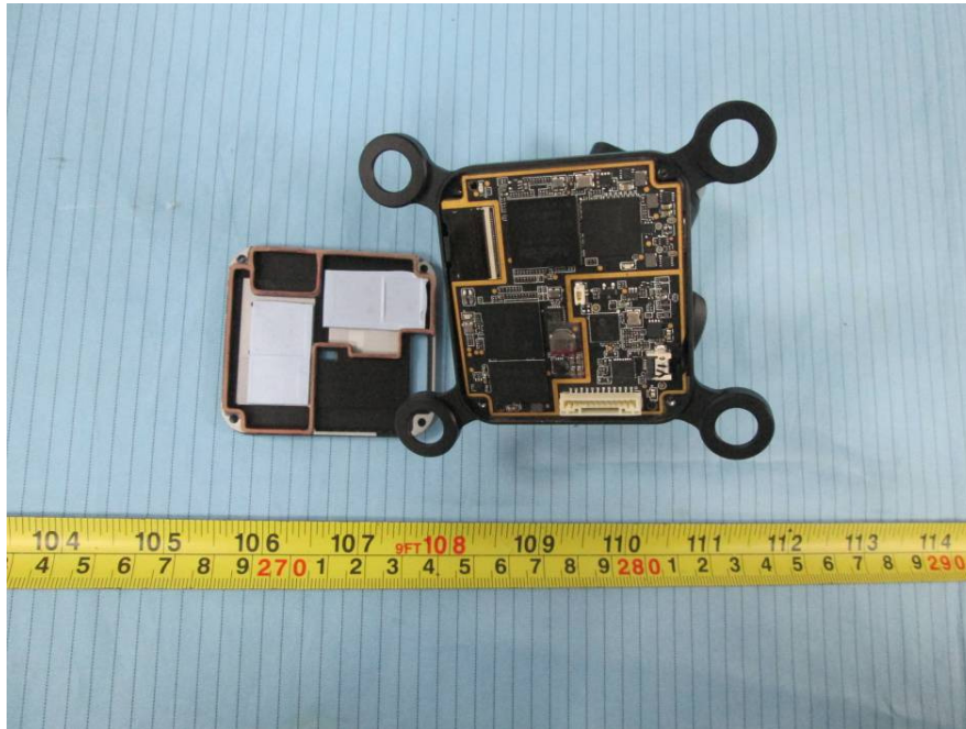
EUT – Pan-Tilt Cover off View 4
