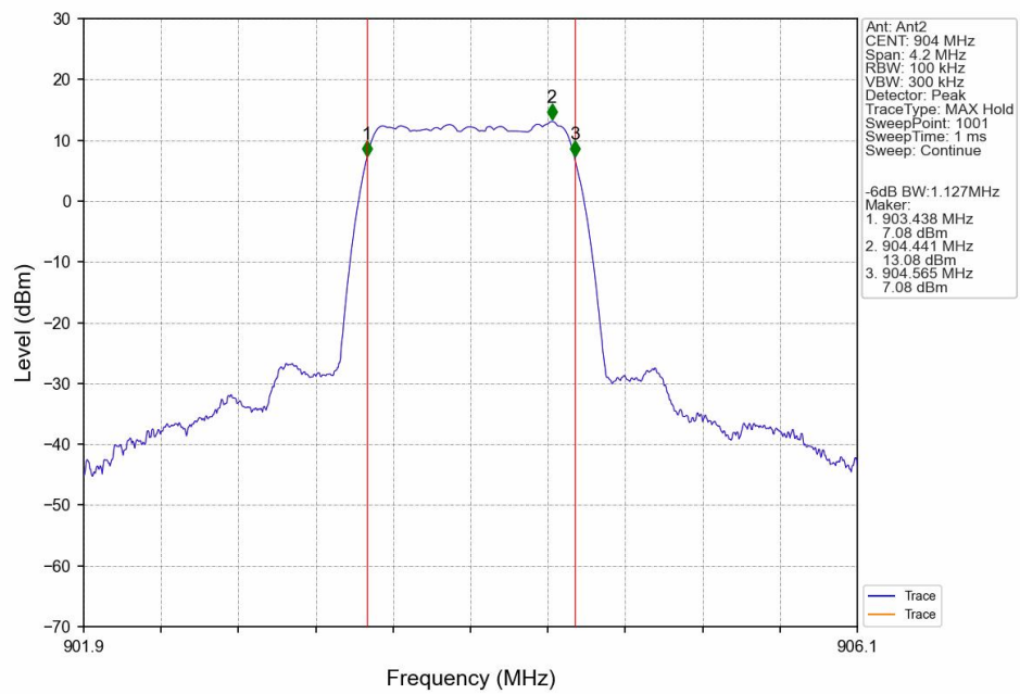
16QAM_LCH_904MHz_Ant2_NTNV
