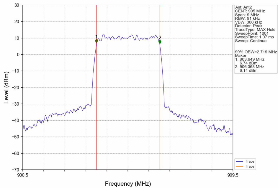
16QAM_LCH_905MHz_Ant2_NTNV
