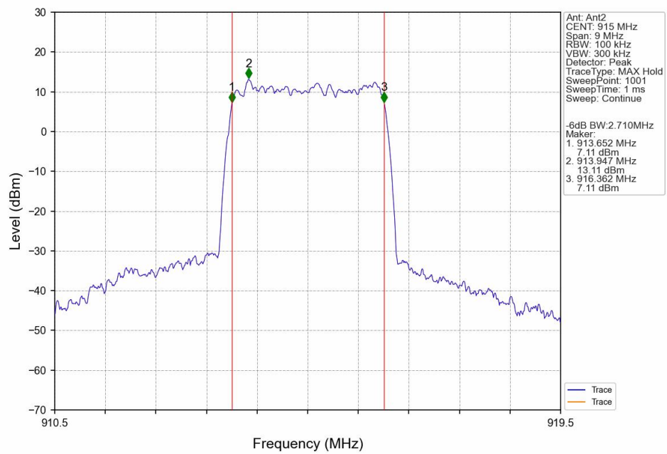
QPSK_MCH_915MHz_Ant2_NTNV
