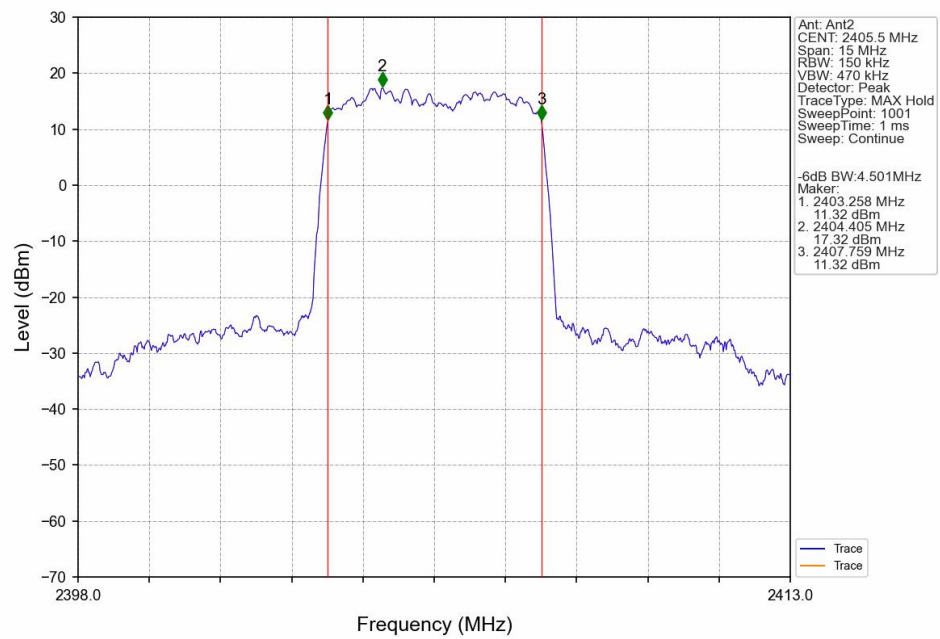
QPSK_LCH_2405.5MHz_Ant2_NTNV
