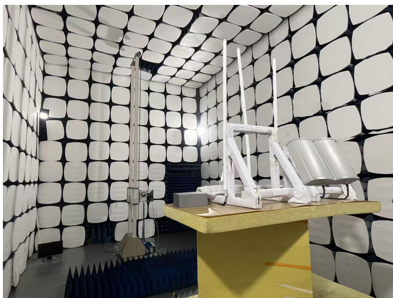
Radiated Spurious Emission, Above 1GHz
