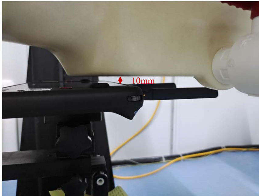
Body Front Setup Photo(10 mm)
