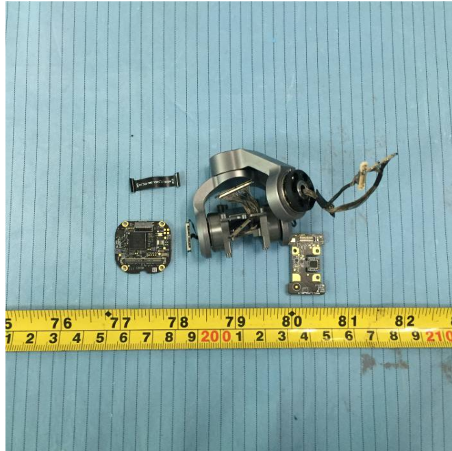
EUT –Camera Cover off View 4
