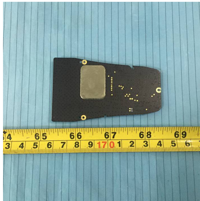
EUT – GPS Board Bottom View
