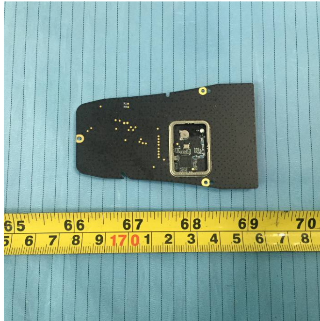
EUT – GPS Board Bottom Shielding off View
