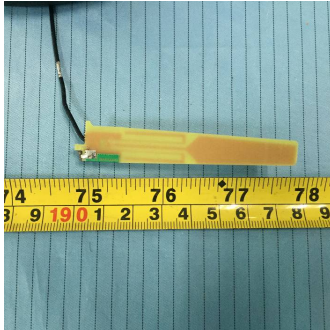
EUT –Antenna 2 Board Bottom View
