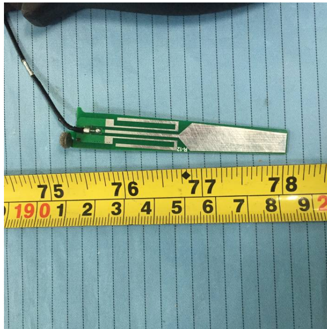
EUT –Antenna 1 Board Top View
