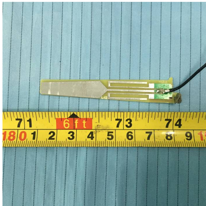
EUT –Antenna 2 Board Top View
