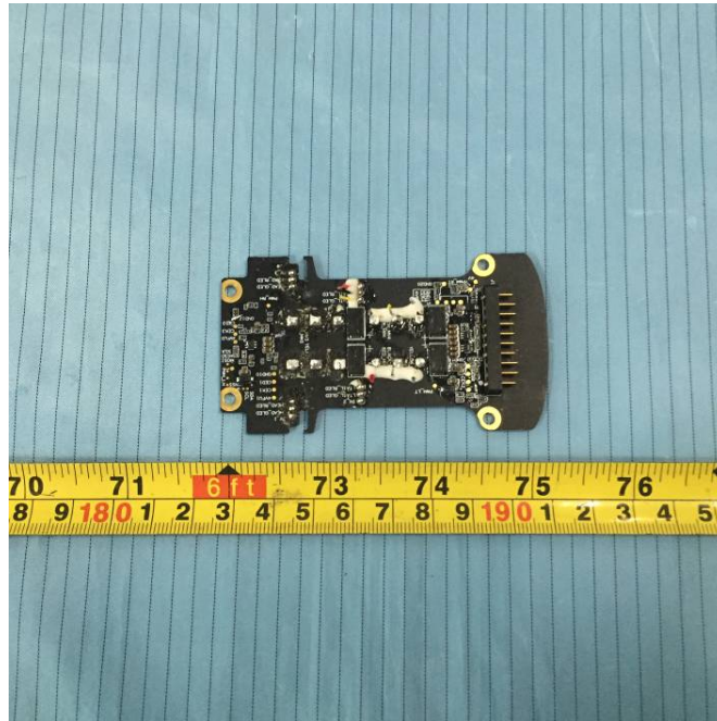
EUT – Main Board 3 Top View
