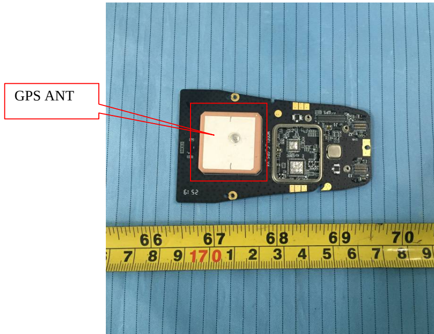
EUT – GPS Board Top Shielding off View
