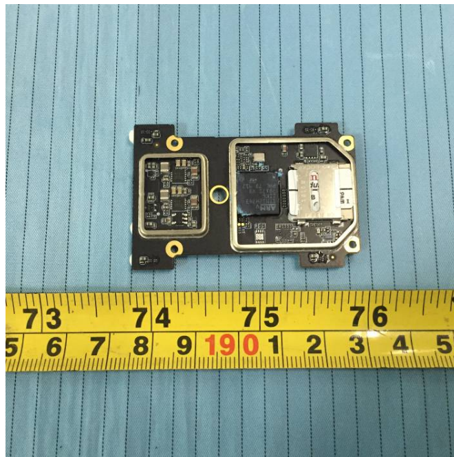
EUT – Main Board 2 Bottom Shielding off View
