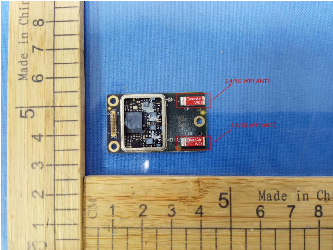
WIFI Chip+ANT
