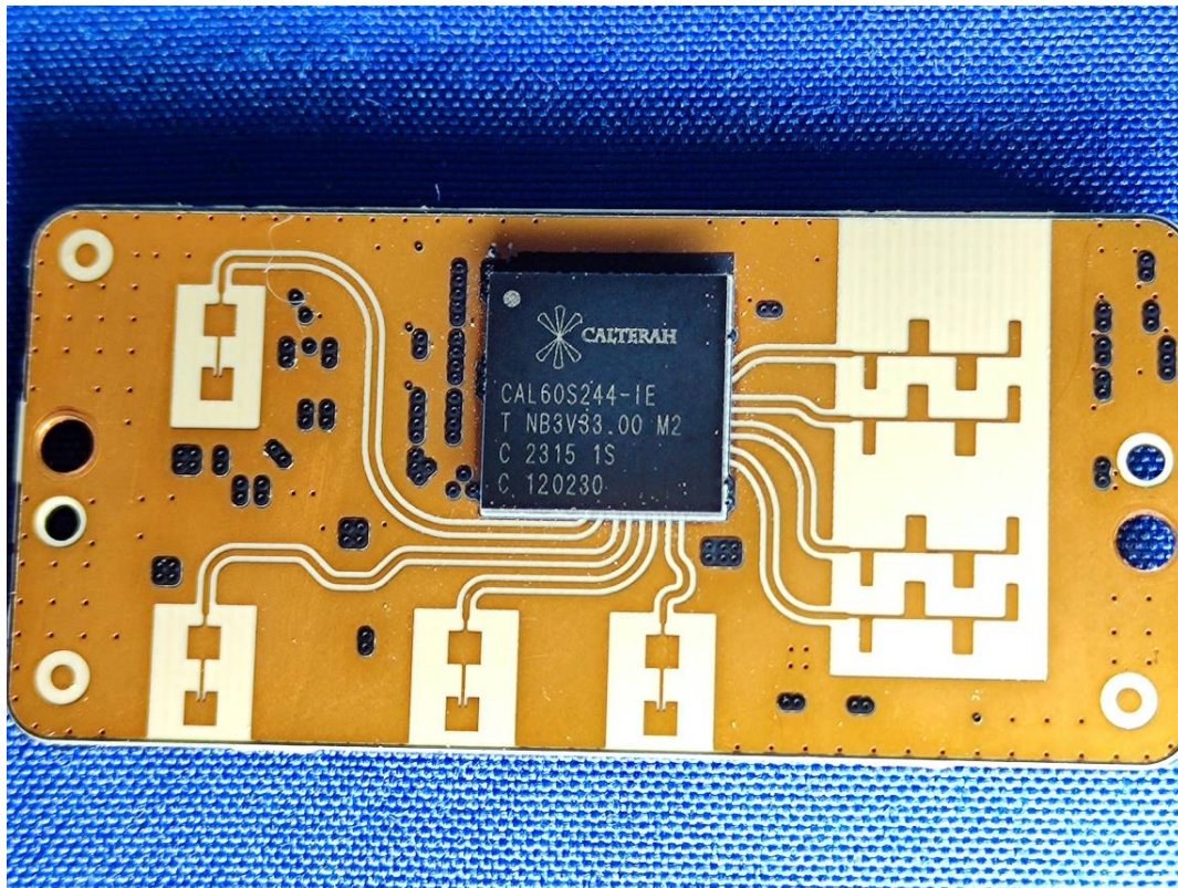
Chip+Antenna
