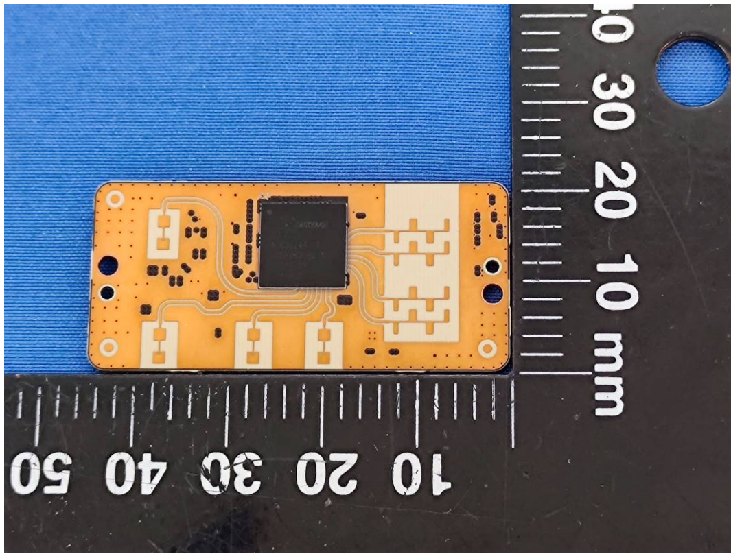
Chip+Antenna
