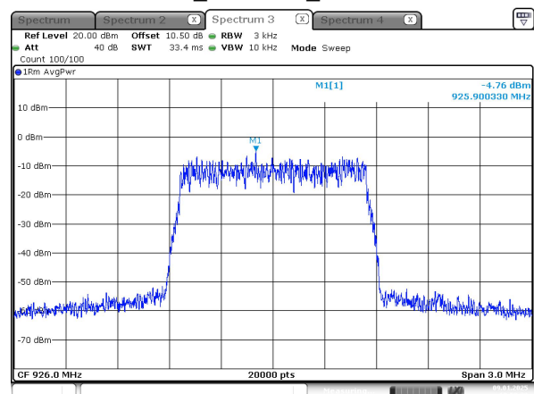
1.4M_926 MHz_Chain 1
