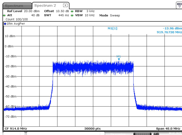
20M_914 MHz_Chain 0
