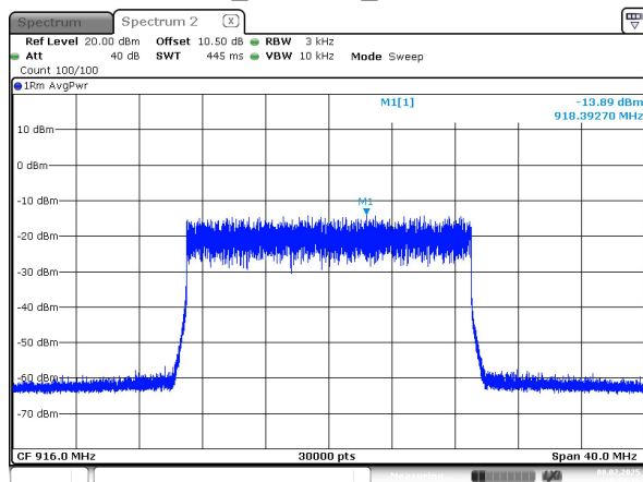
20M_916MHz_Chain 0
