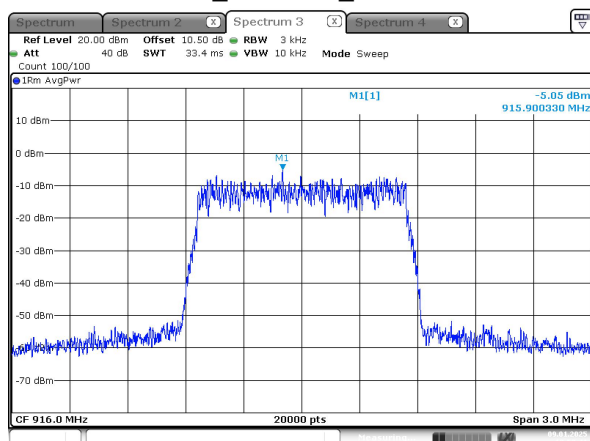
1.4M_916 MHz_Chain 1
