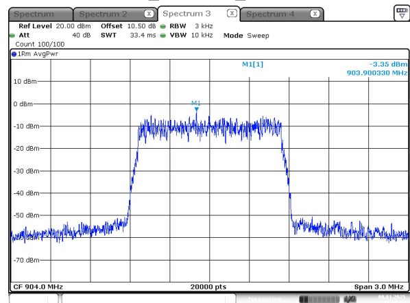
1.4M_904 MHz_Chain 1
