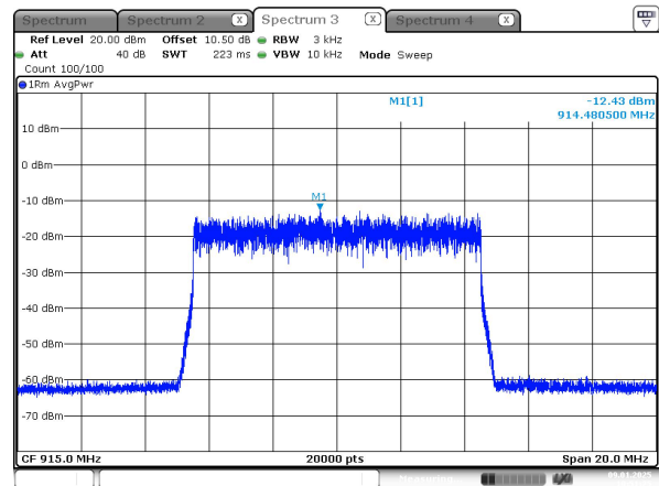
10M_915 MHz_Chain 1
