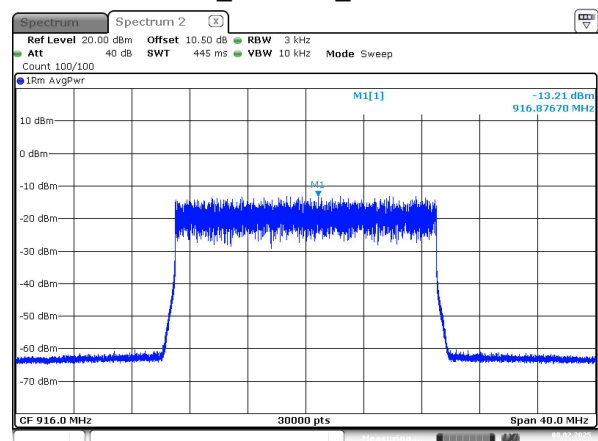
20M_916MHz_Chain 1
