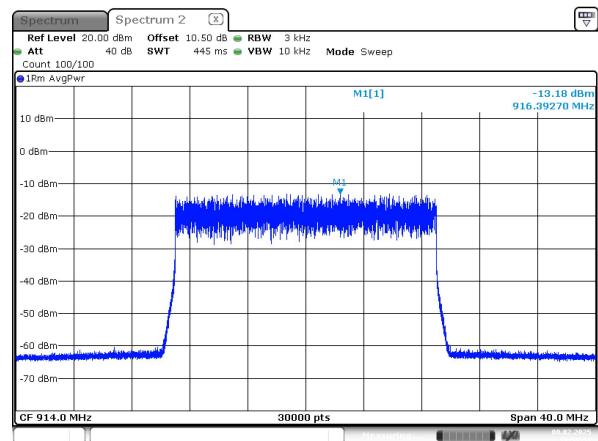
20M_914 MHz_Chain 1
