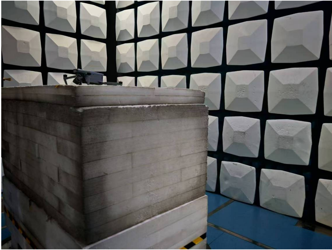
Radiated Emission 140-200GHz View
