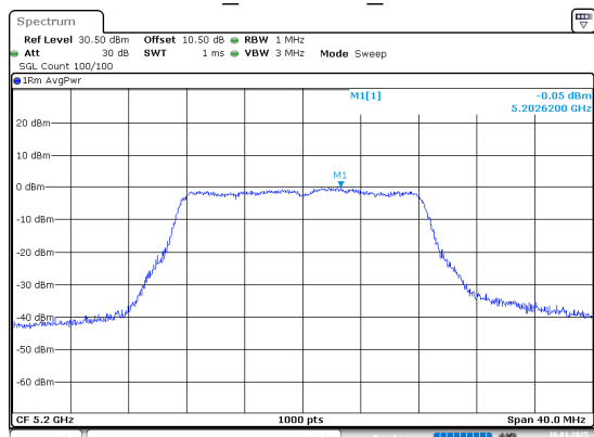
802.11a_5200MHz_Chain 1
