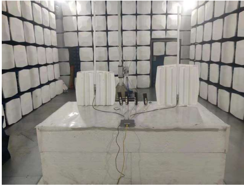
Above 1GHz
