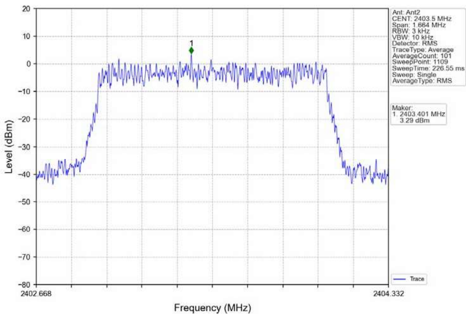
16QAM 1.4MHz_LCH_2403.5MHz_MIMO_NTNV
