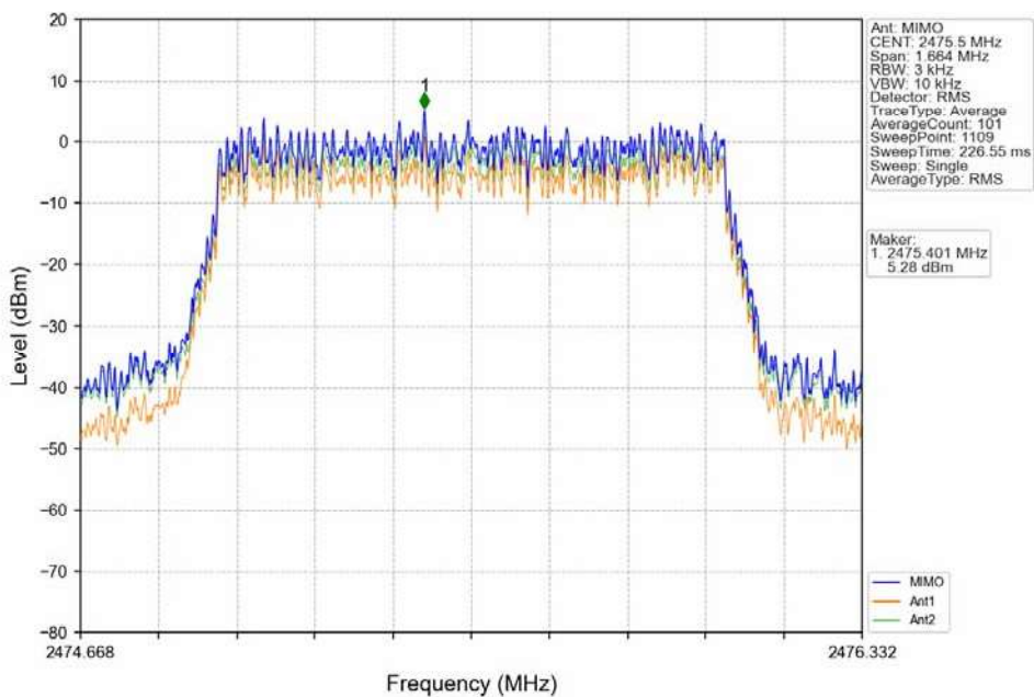
16QAM 1.4MHz_HCH_2475.5MHz_MIMO_NTNV
