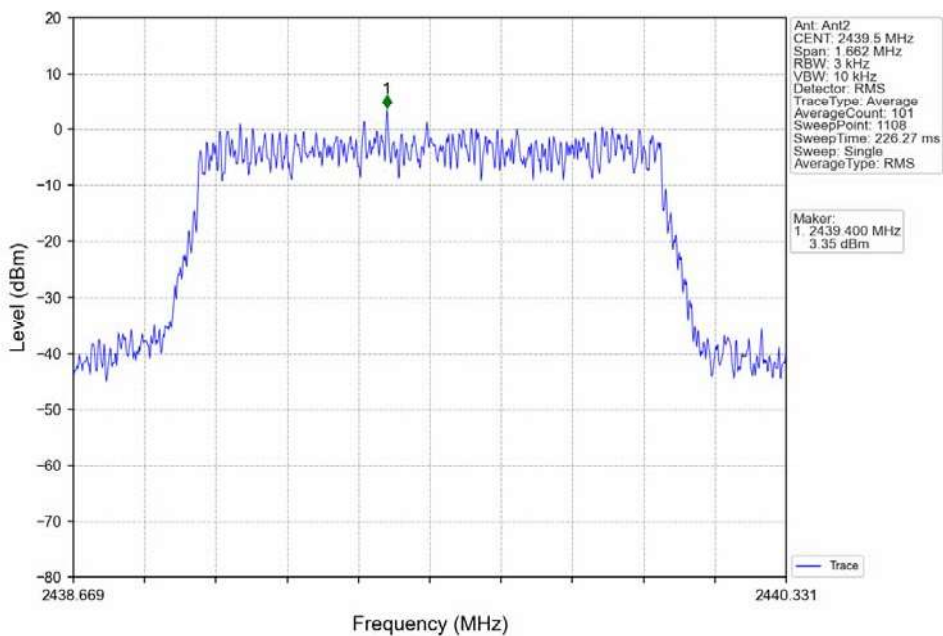
16QAM 1.4MHz_MCH_2439.5MHz_Ant2_NTNV
