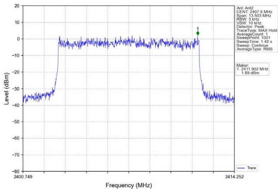
16QAM 10MHz_LCH_2407.5MHz_MIMO_NTNV
